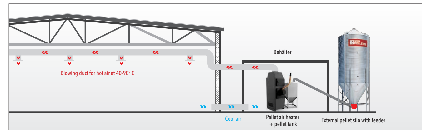
Air heating with external pellet silo and heater container
