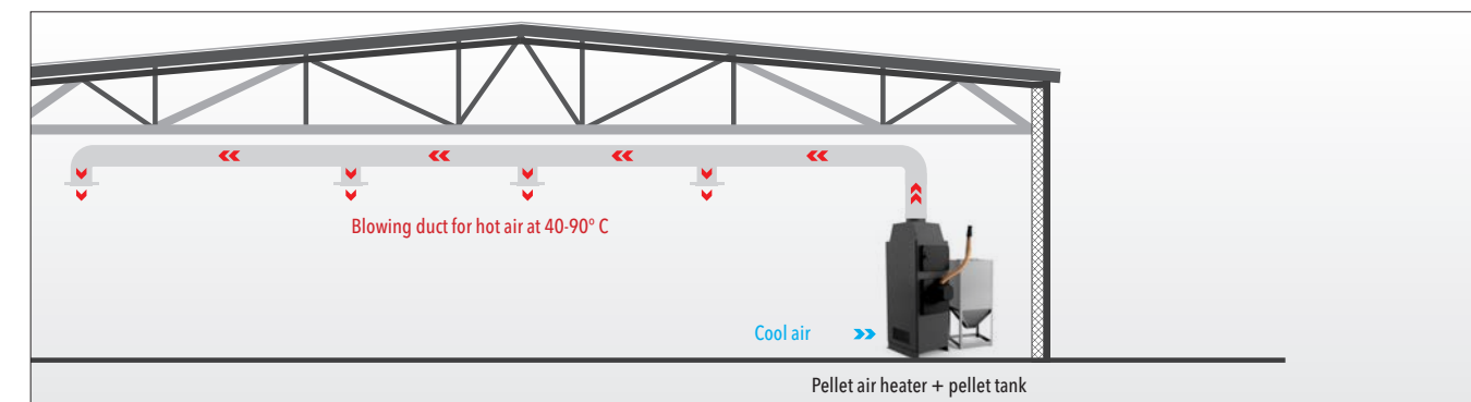
Air heating with integrated pellet tank 400 L
